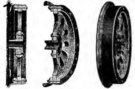
Figs. 5629-5631. THE SHEFFIELD HAND-CAR WHEEL. Hub and Rim of Steel, Wood Felloe and Spokes.
